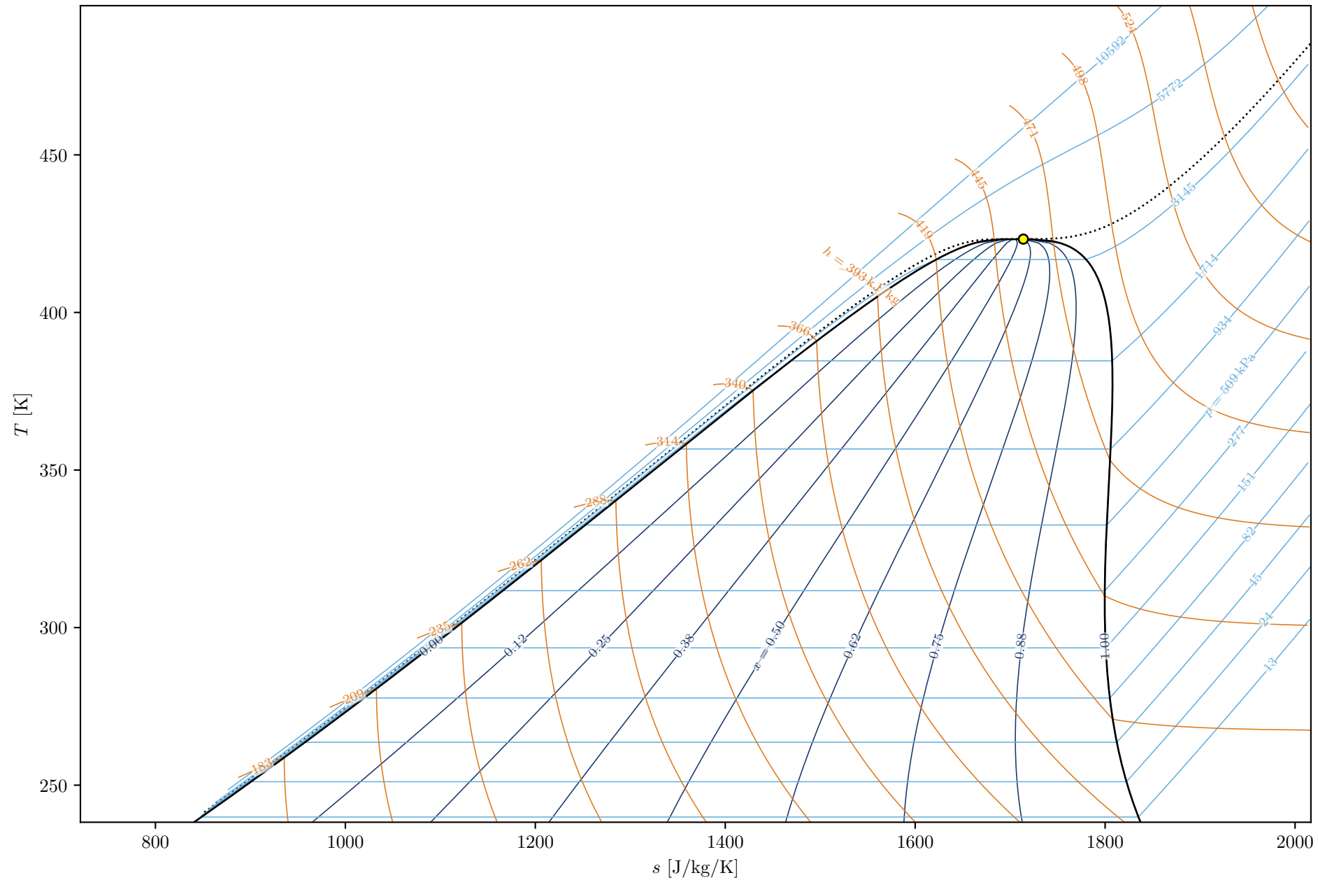
Thermodynamic Diagram (TS) — R1234ze(Z)
